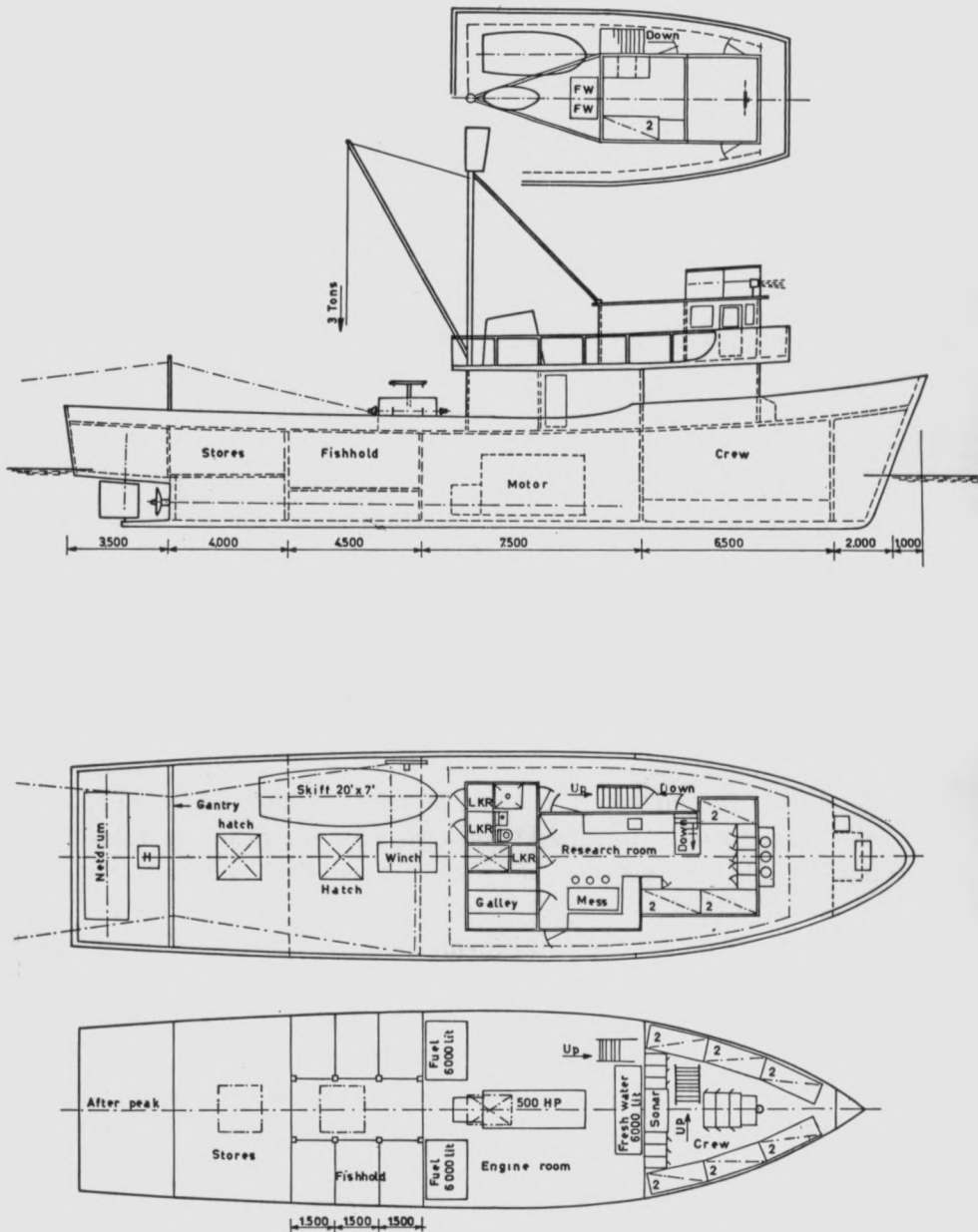
Fig. 3 — Research vessel 29.00 x 7.000 x 3.200 m.
