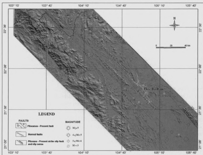
Fig. 3. — Active fault segments along Red River faults and Chay River fault.
