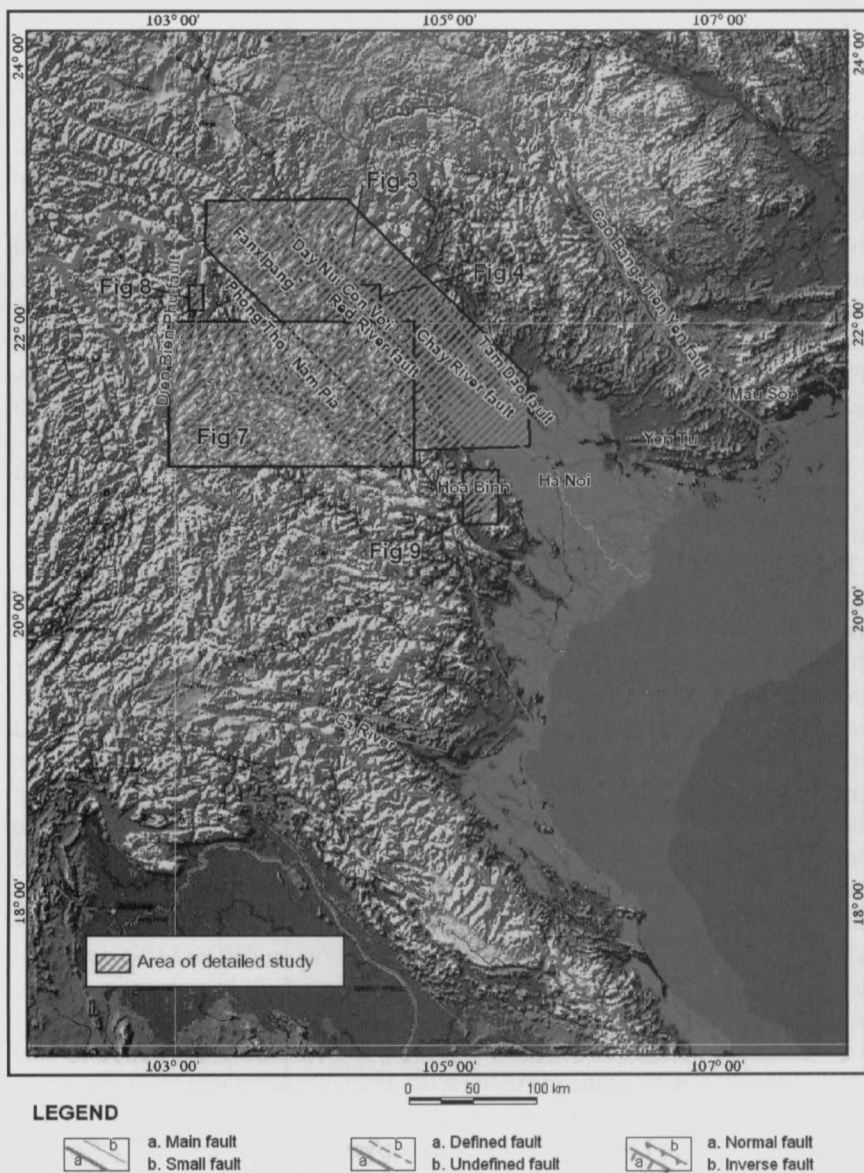
Fig. 2. — Active faults in North Vietnam and area of detailed study.
