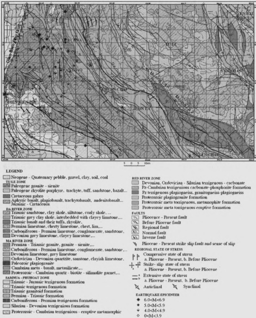
Fig. 7. — Seismotectonic map of Son La hydropower dam area.
